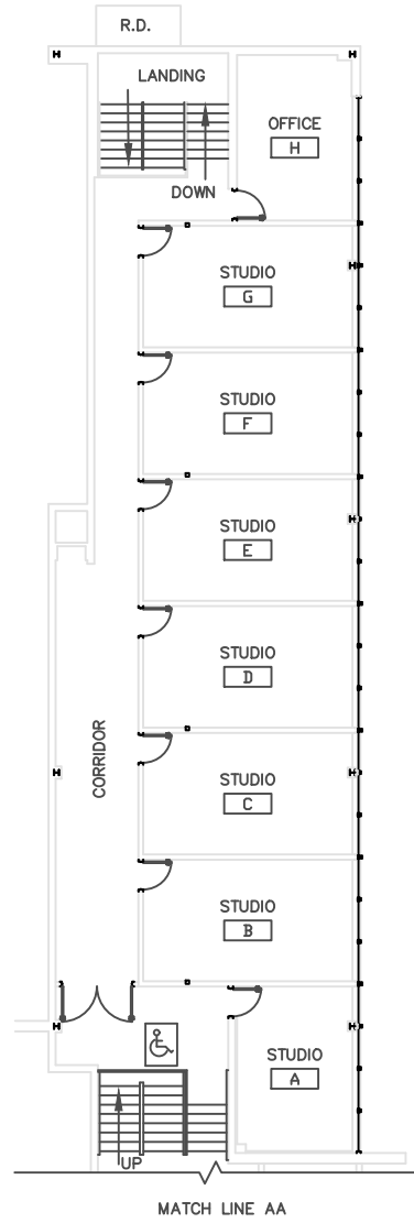
MEZZANINE FLOOR PLAN SCALE : 1" = 20'
